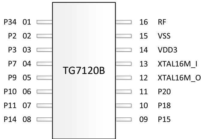
Figure 2: Pin assignment – TG7120B SOP16 package
