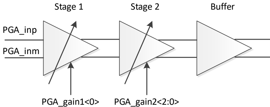
Figure 16: PGA path
