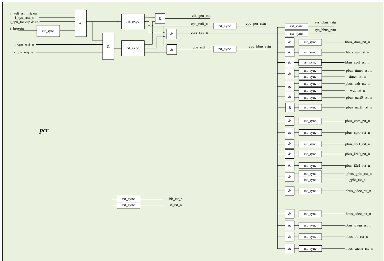
Figure 6: TG7120B power, clock and reset
