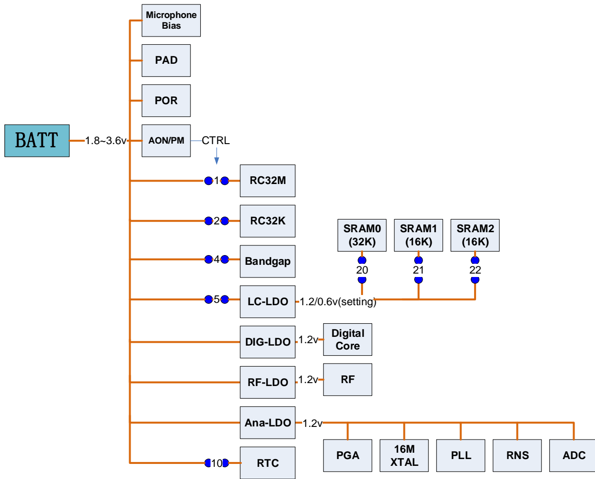
Figure 7: Power system
