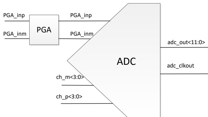
Figure 15: ADC
