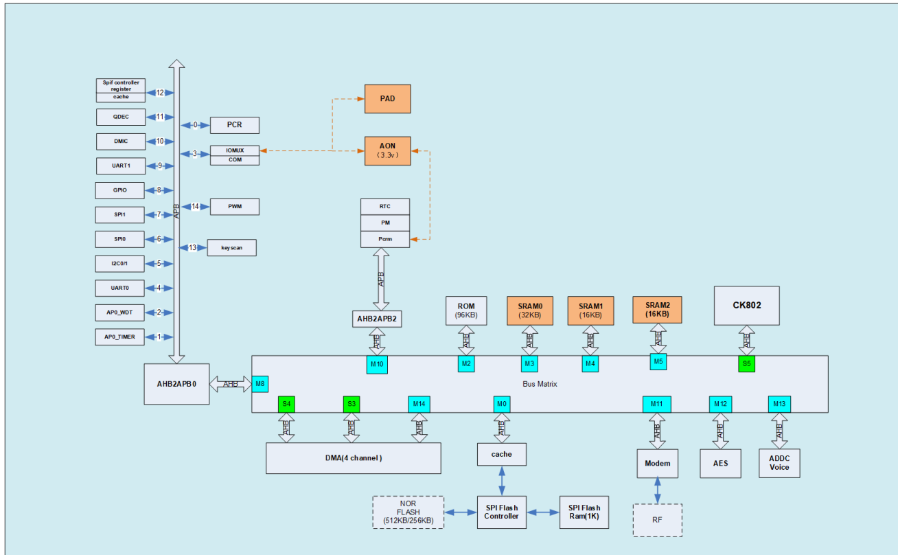
Figure 1: TG7120B block diagram
