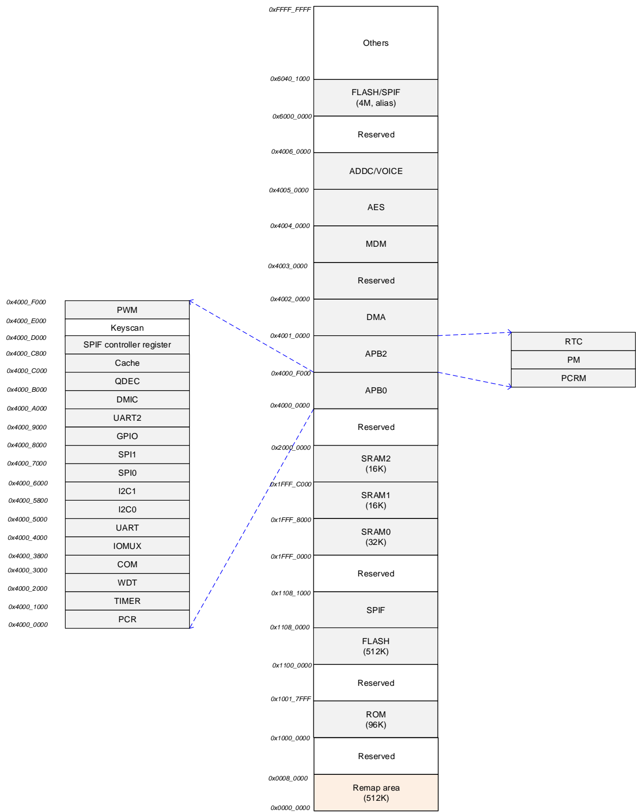
Figure 3: TG7120B memory space
