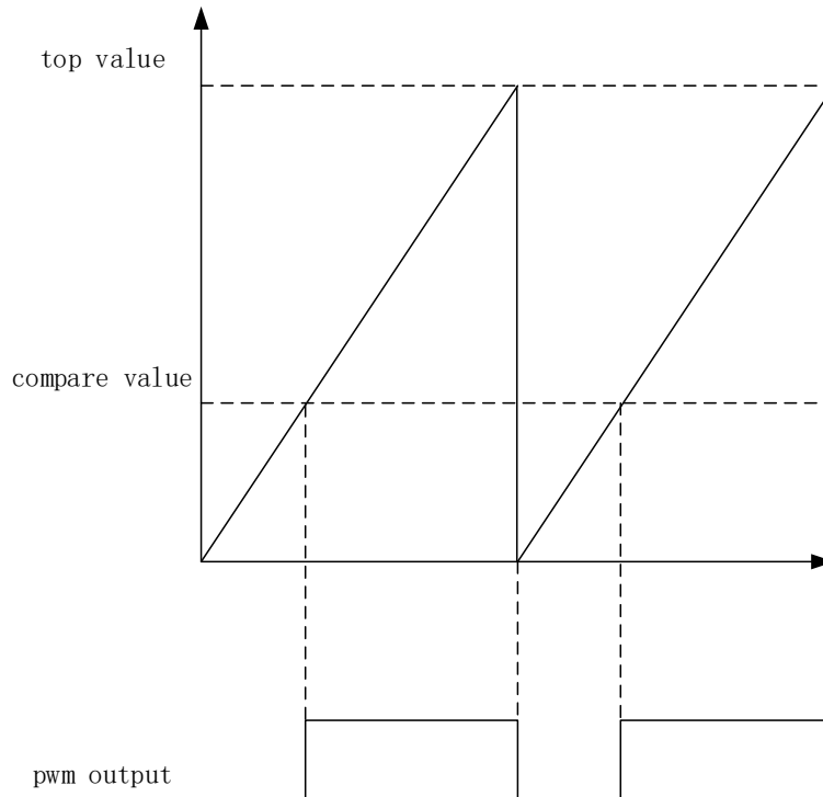
Figure 14: PWM operation
